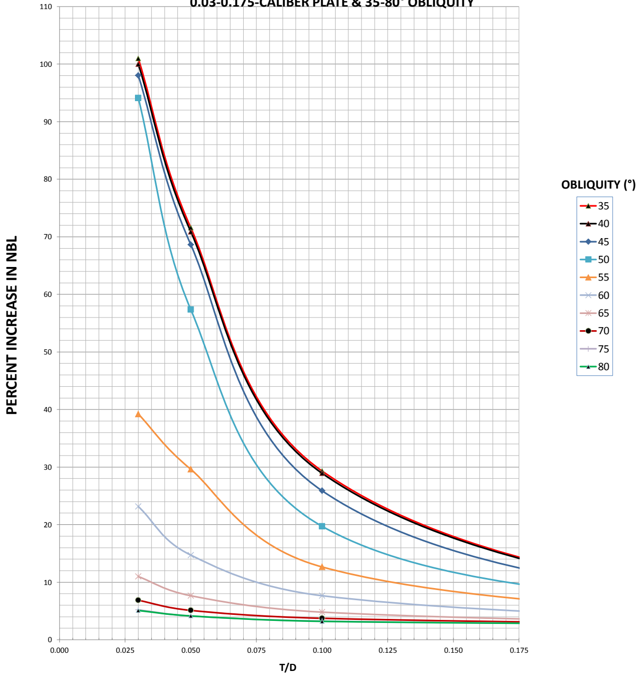
5% WINDSCREEN EFFECT ON NBL DETAILS: 0.03-0.175-CALIBER PLATE & 35-80° OBLIQUITY
