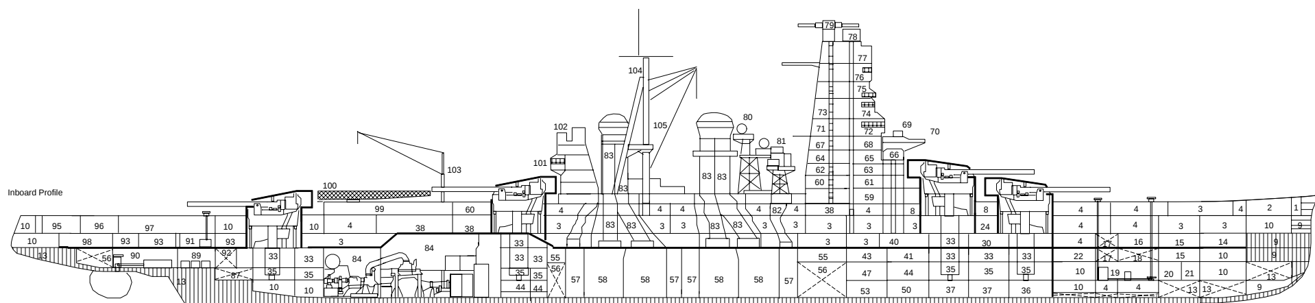
Inboard Profile
