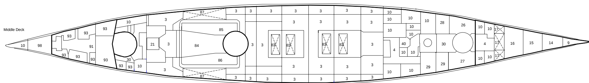
Middle Deck
